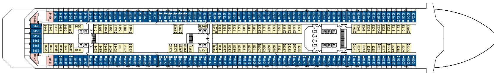
DECK 8 - PERSEUS
