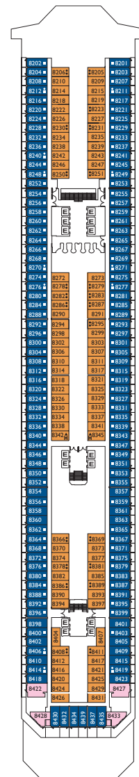
DECK 8 VERONESE
