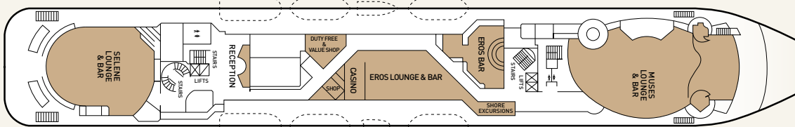
DECK 5 - DIONYSSOS
